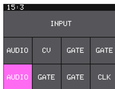
Input Settings
