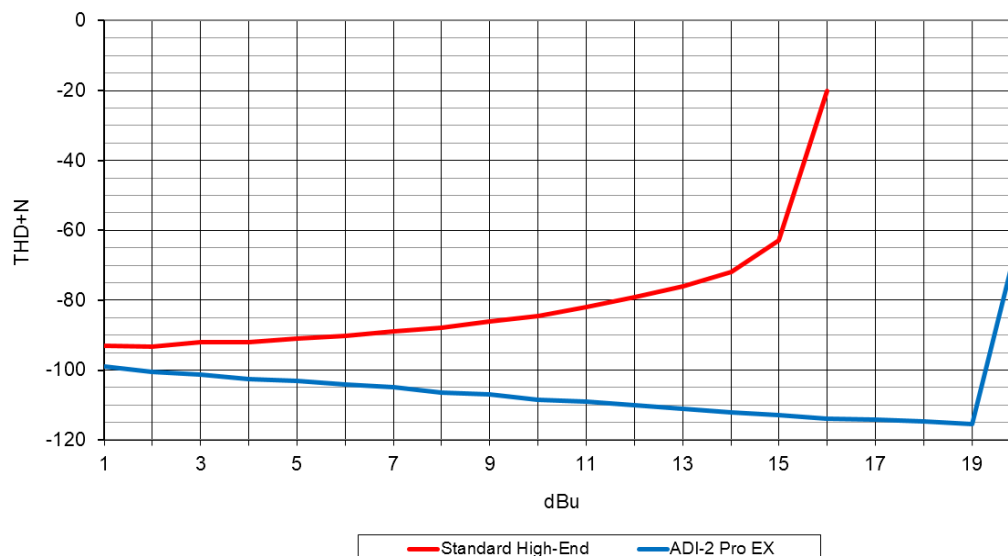
Phones Out THD+N @ 32 Ohm Load
