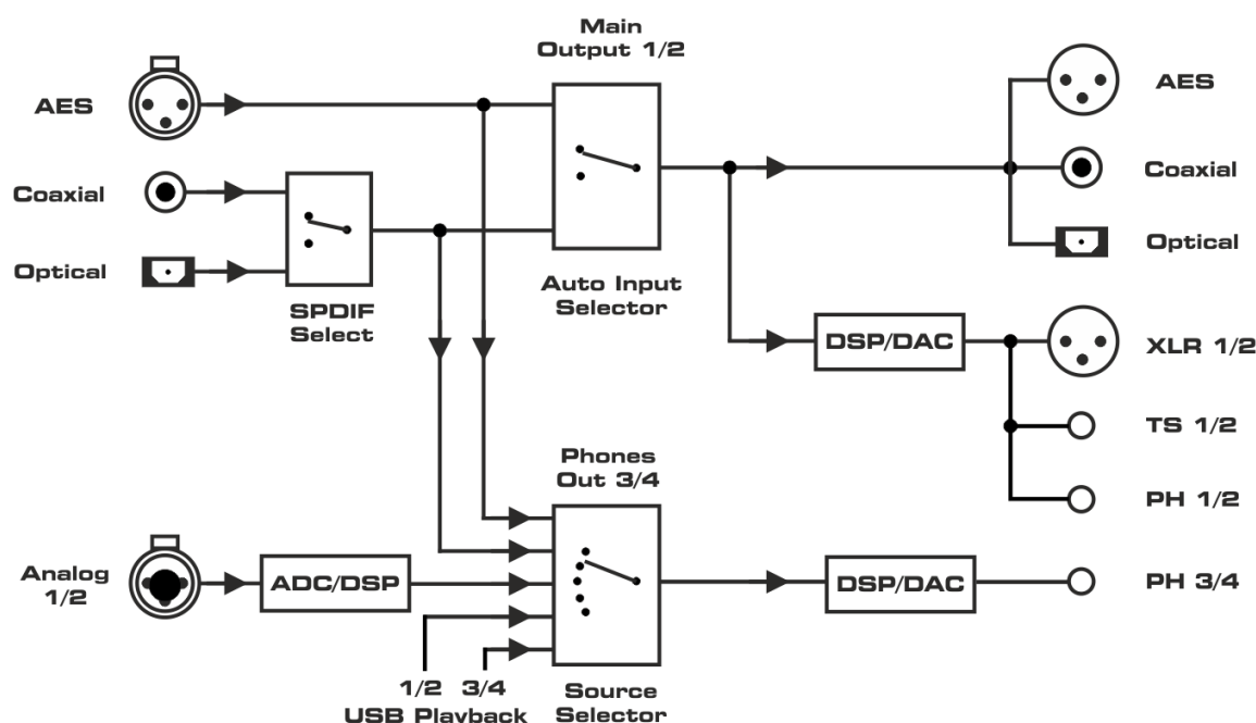
ADI-2 Pro Digital Thru Mode (with Monitoring)
